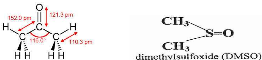
Figure 1. Molecular structure of Acetone and DMSO
